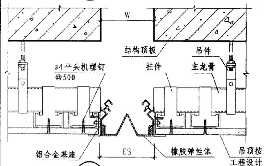
③ 吊顶 (QTT-2)
