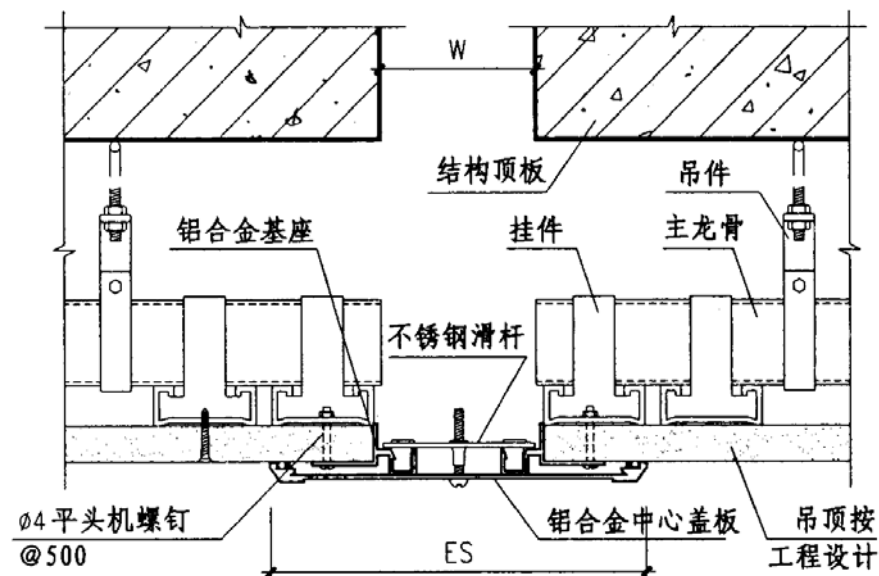
③ 吊顶 (QBH)
